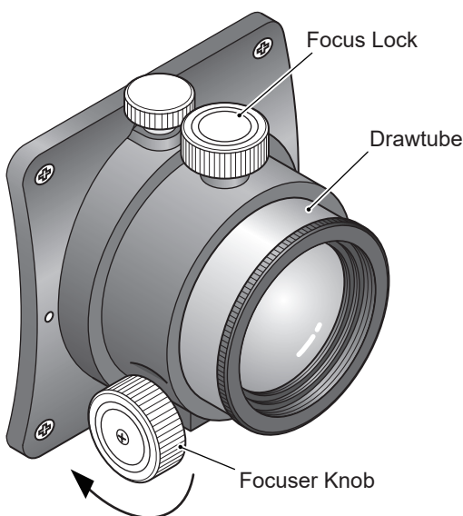
Rotating in this direction moves the draw tube outward
