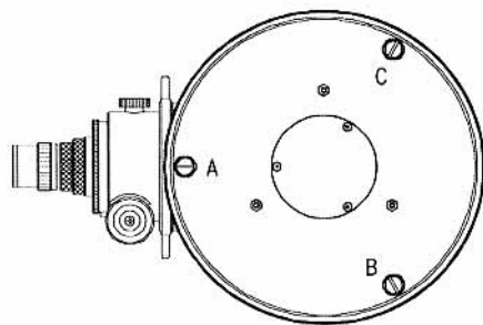
Primary mirror adjusting screw; A, B, C.
